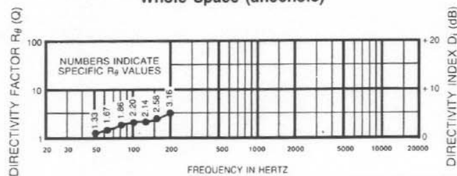
FIGURE 4 — MTL-2 Directivity Factor R_{\theta} (Q) and Directivity Index D_1 vs. Frequency Whole Space (anechoic)
