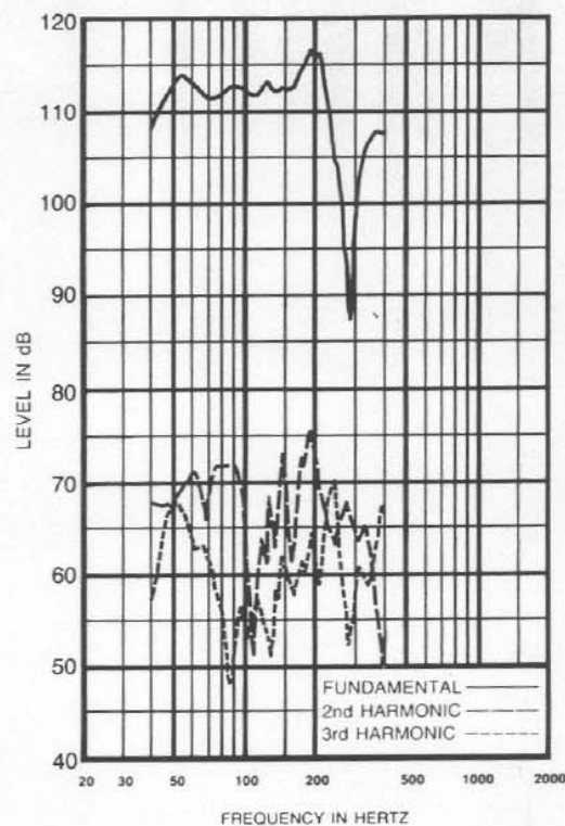
FIGURE 5 — MTL-2 Harmonic Distortion, 0.1 Rated Power Input (80 watts), 10 Feet on Axis
